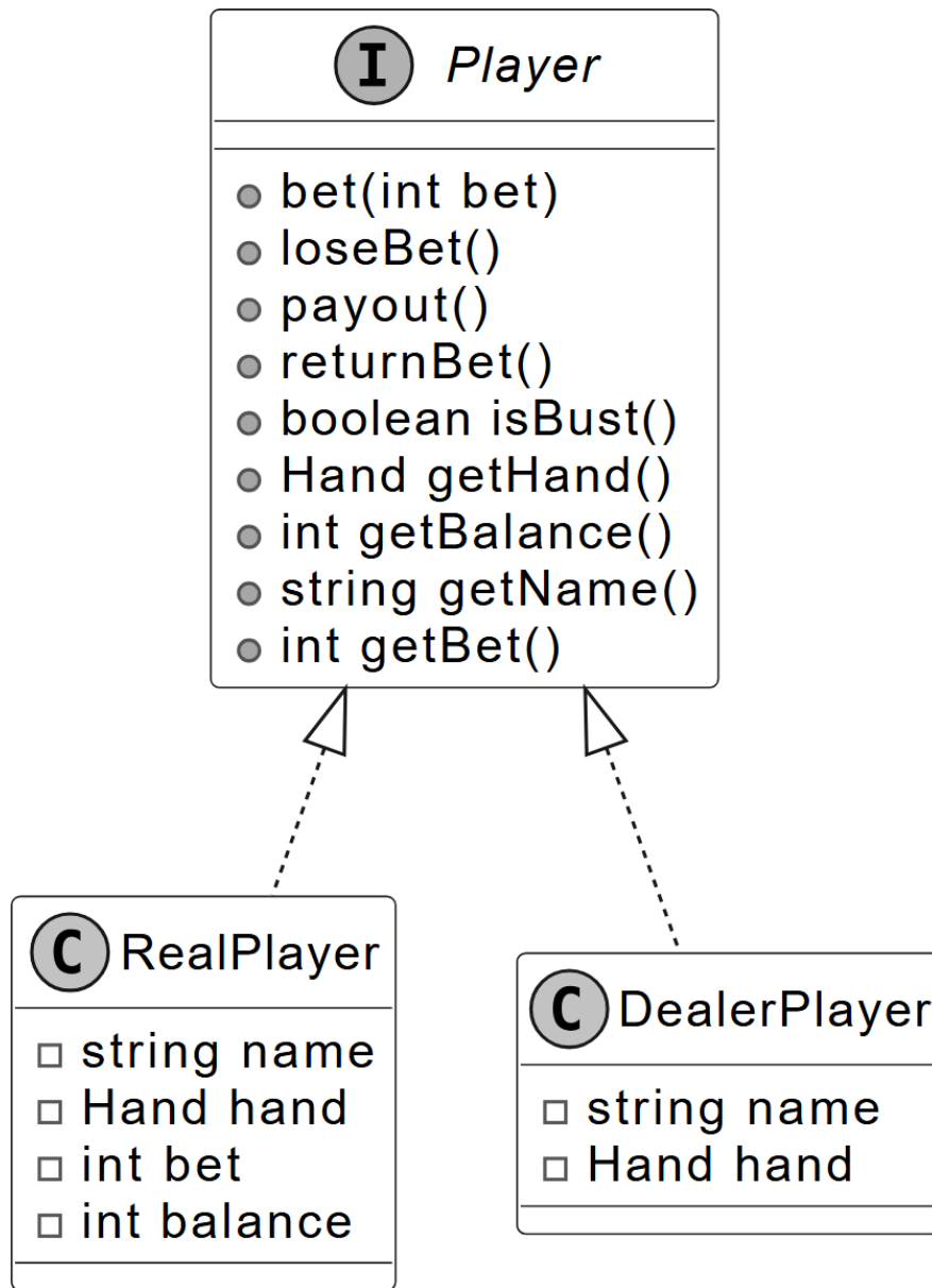
Player interface with concrete classes
