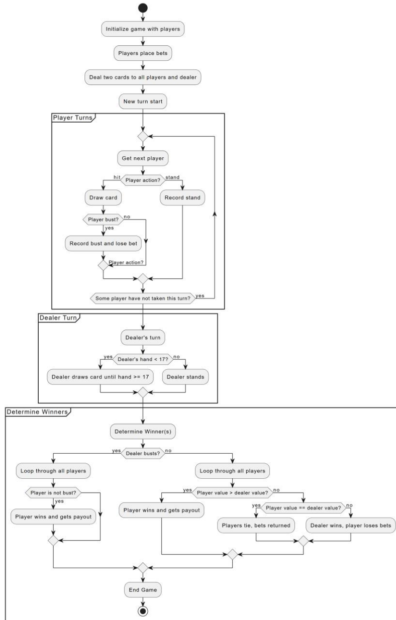
Activity Diagram of Blackjack Game
