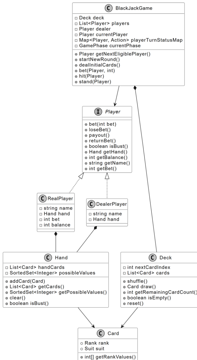
Class Diagram of Blackjack
